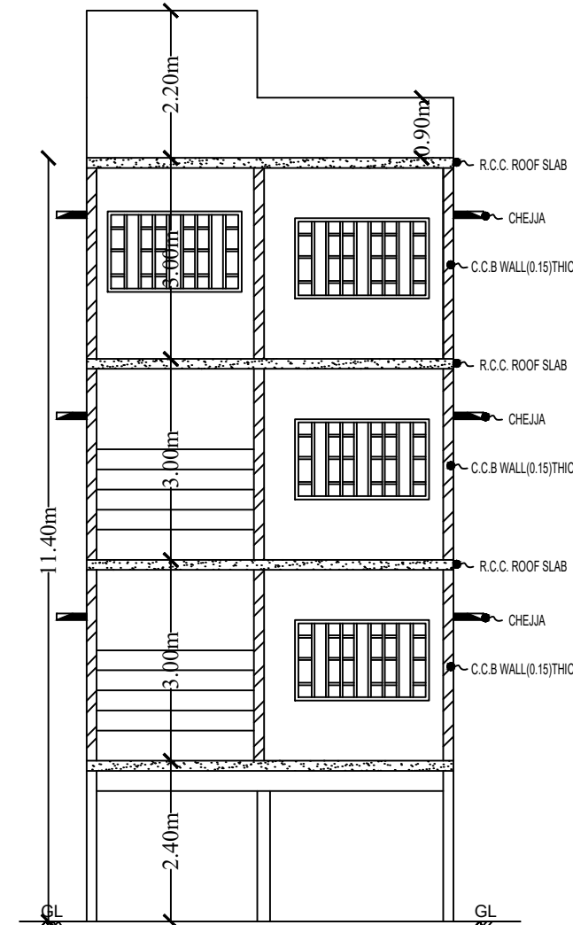
SECTION @ A-A
