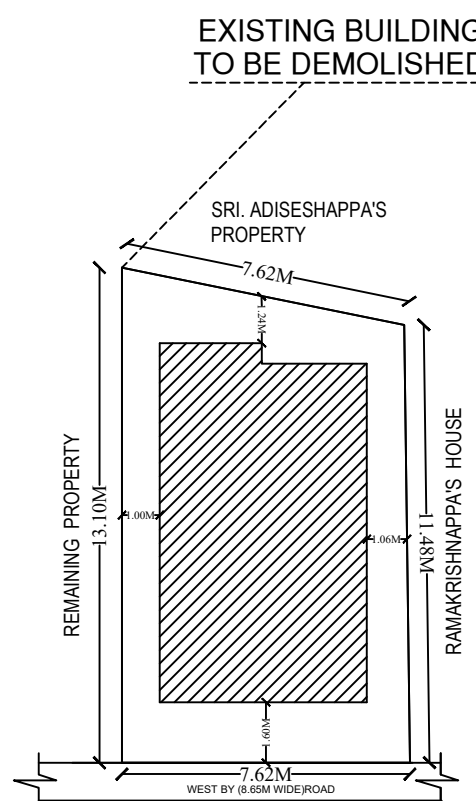
SITE PLAN
